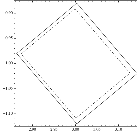
Figure 1: Inner approximation of the range of a vector-valued function.
